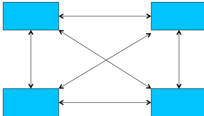
FIGURE 1 – Architecture logicielle
